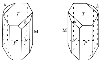
Figure 2 Simplified form of hemihedral crystals of sodium ammonium tartrate according to Pasteur.
