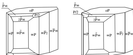
Figure 1 Sketches of the hemihedral crystals of sodium ammonium tartrate according to Kekulé.
